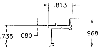
4 GLASS STOP (3/8" GLASS)
