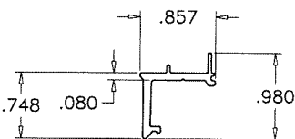
4 GLASS STOP (3/8" GLASS)
